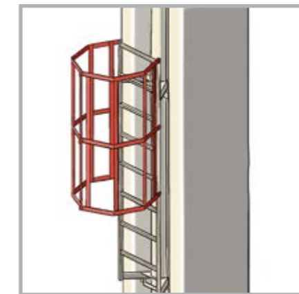
Ladder element with removable back protection
